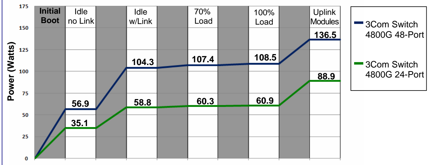
Figure 2: 3Com Switch 4800G 24-Port and 48-Port Power Profile
