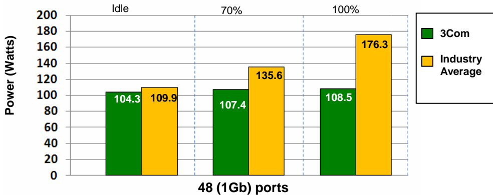
Figure 4: 3Com Switch 4800G 48-Port Power Consumption
