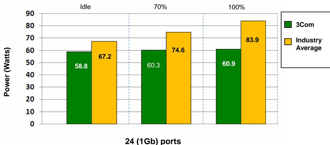
Figure 3: 3Com Switch 4800G 24-Port Power Consumption
